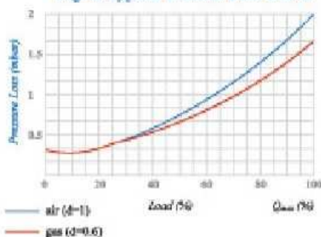
Fig. 2: Typical Pressure Loss Curve
