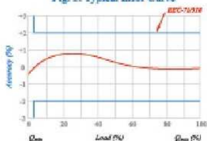
Fig. 3: Typical Error Curve
