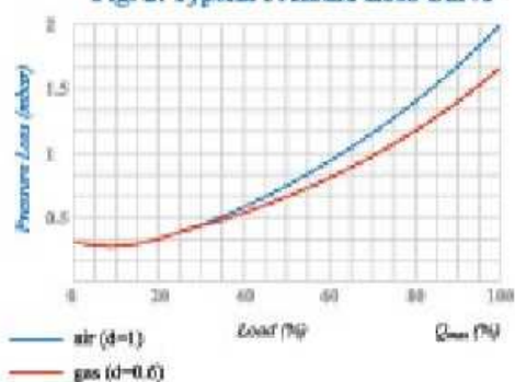
Fig. 2: Typical Pressure Loss Curve
