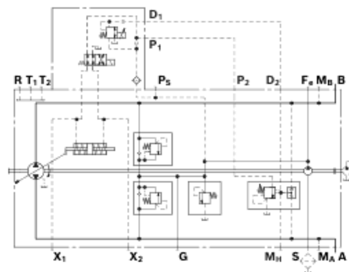
▼ Circuit diagram, standard version ED4
