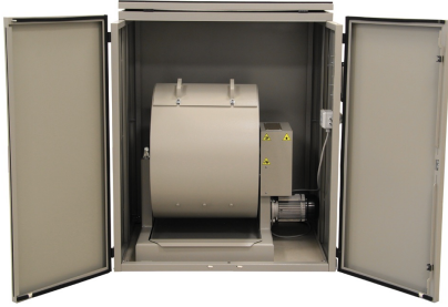
Los Angeles abrasion machine model 48-D0500/G with noise reduction and CE compliant safety cabinet model 48-D0500/CB2
