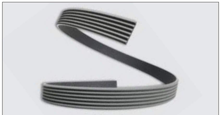
Example of belts with clefts welded on the back. Many different types of cleft are available
