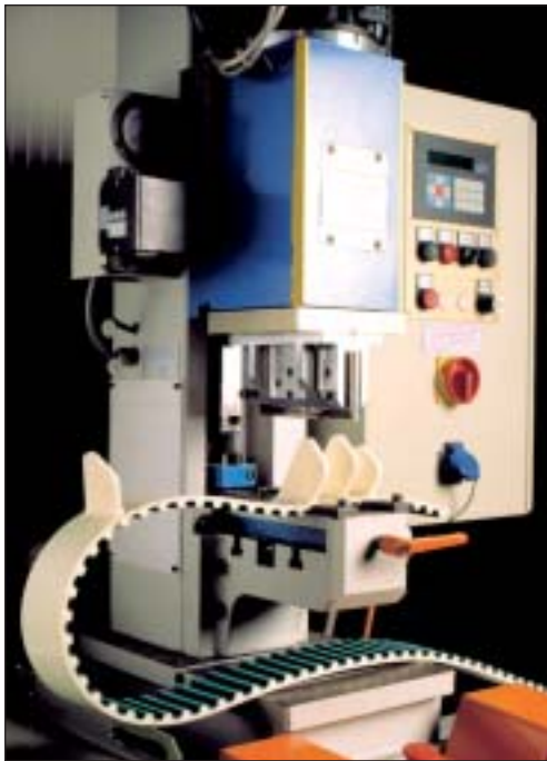
Cleft welding machine
