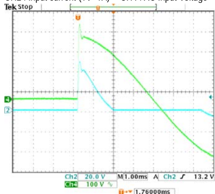
INPUT=230VAC/50HZ @ FULL LOAD CH2 : Input current (1V=1A) CH4 : AC Input Voltage
