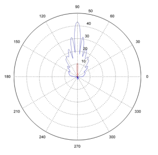
5.5 Ghz E-Plane and H of E-plane
